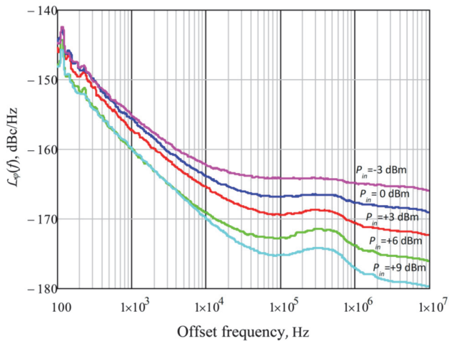
Figure 7 Measured residual phase noise of 1.57 GHz SAW resonator.
