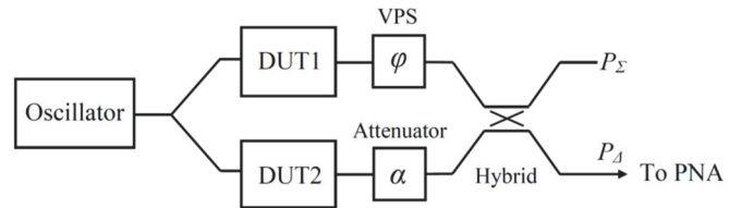
Figure 3 Dual DUT PNA-based noise measurement system using interferometric method.
