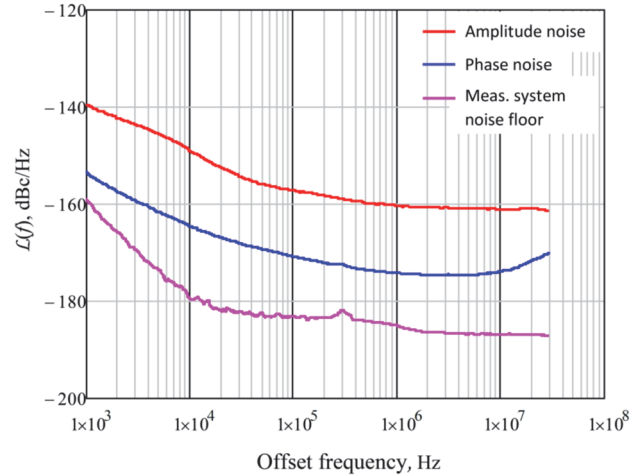
Figure 5 Measured residual noise of Qorvo CMD275 MMIC amplifier ( f = 6.4 GHz).
