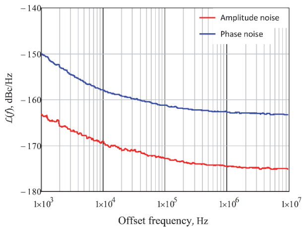
Figure 8 Measured residual amplitude and phase noise of times four frequency multiplier.
