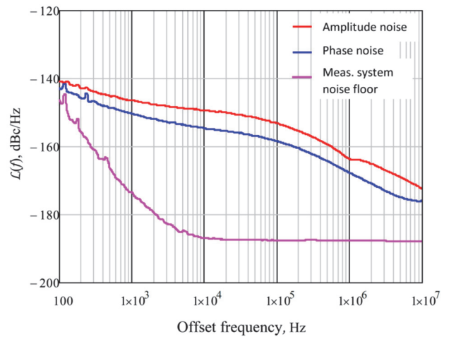
Figure 6 Measured residual noise of Analog Devices HMC8410 MMIC amplifier ( f = 6.4 GHz).
