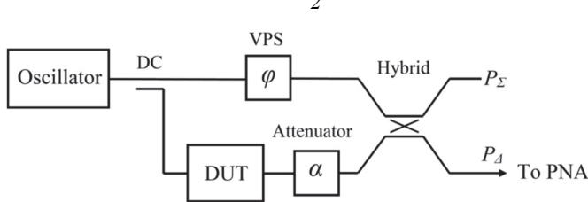
Figure 2 PNA-based noise measurement system using interferometric method.
