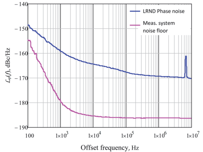
Figure 9 Measured residual phase noise of 6.4 GHz LNRD.
