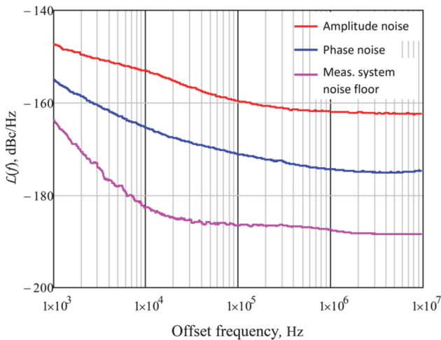
Figure 4 Measured residual noise of Analog Devices HMC606 MMIC amplifier ( f = 6.4 GHz).
