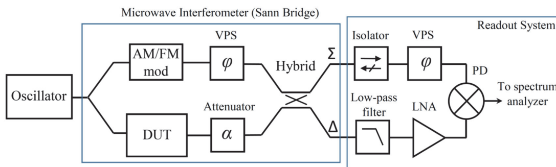
Figure 1 Traditional interferometric noise measurement system.
